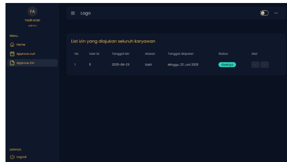
Gambar 10 Dashboard Admin
