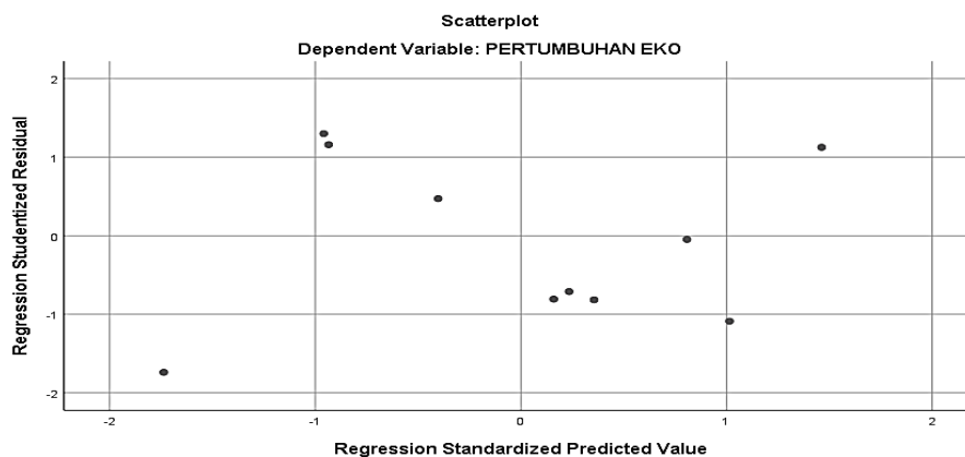
Gambar 1. Scatterplot
