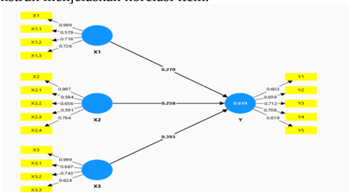
Gambar 3. Diagram Jalur Model
