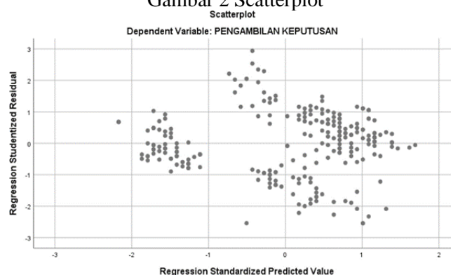
Gambar 2 Scatterplot
