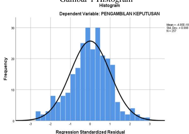
Gambar 1 Histogram
